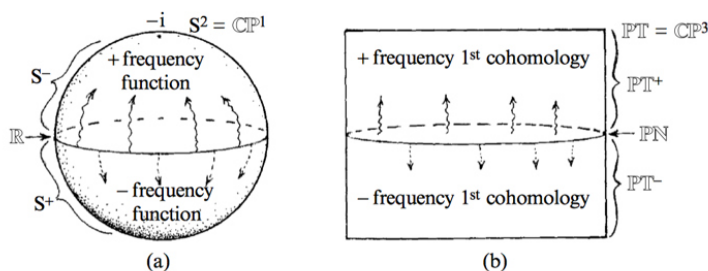
FIGURE 6. — An analogy between the Riemann sphere S^2(= \mathbb{CP}^1) and projective twistor space \mathbb{PT}(= \mathbb{CP}^3) . (a) A complex function (i.e. a ‘0th cohomology element’), defined on the real axis \mathbb{R} of S^2 , splits into its positive frequency part, extending holomorphically into what is here depicted as the northern hemisphere S^- , and its negative frequency part, extending into the southern hemisphere S^+ . (b) A 1st cohomology element, defined on \mathbb{PIN} (and representing a massless field) splits into its positive frequency part, extending holomorphically into the top half \mathbb{PT}^+ of projective twistor space, and its negative frequency part, extending into the bottom half \mathbb{PT}^- .
